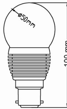
Fig 3. B22 Base
